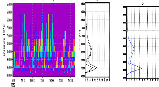
Stochastic Forcing
